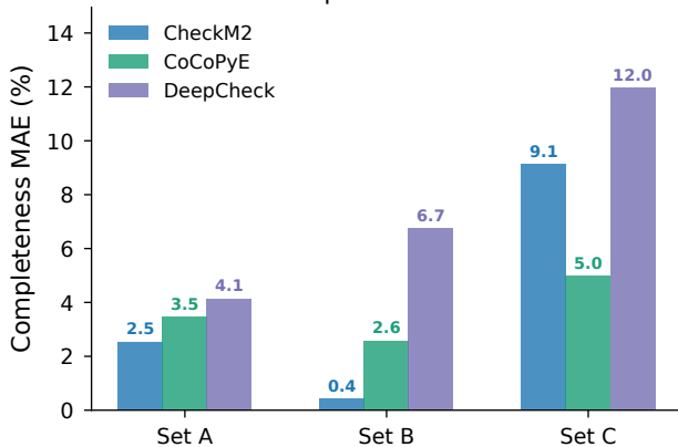
b Completeness MAE
