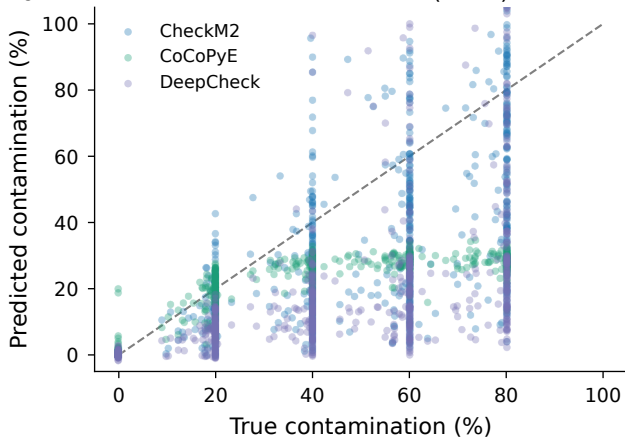
d Pred. vs. true cont. (Set B)
