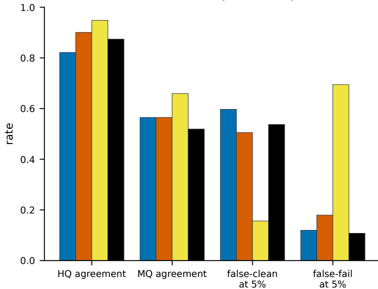
CAMI II marine (mixed bins)
