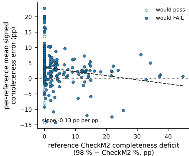
MAGICC v5 (independent)
