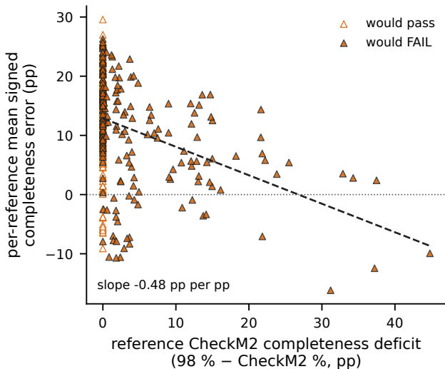
CheckM2 (circular)
