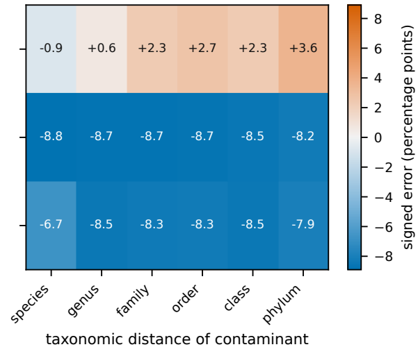
DeepCheck
