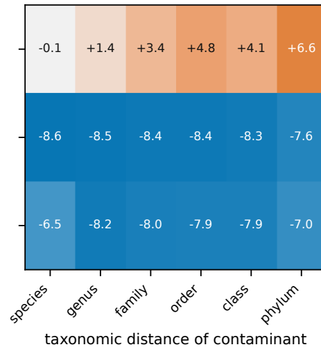
CheckM2 1.0.1
