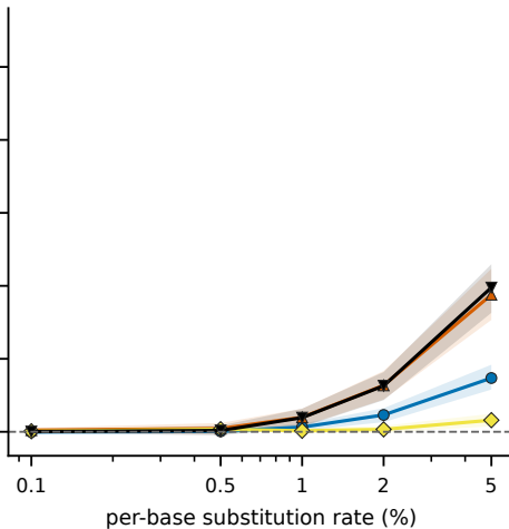
Substitutions (Ti/Tv = 2)
