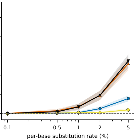
Substitutions (uniform)
