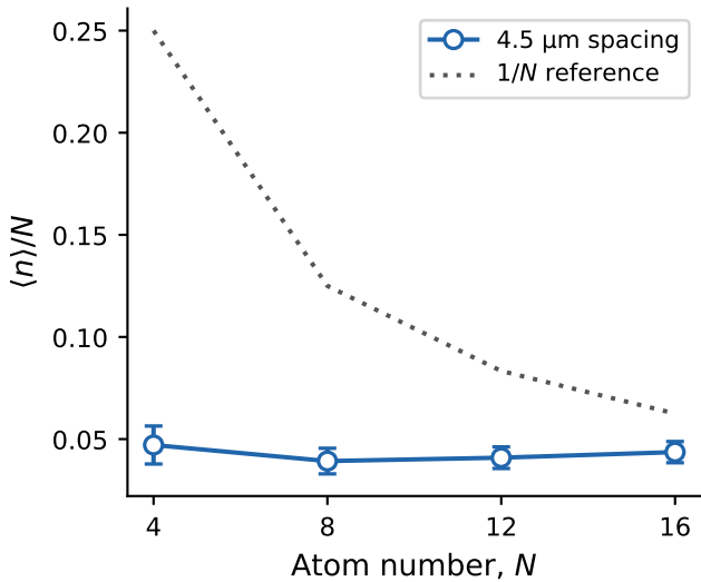
Atom-number scaling
