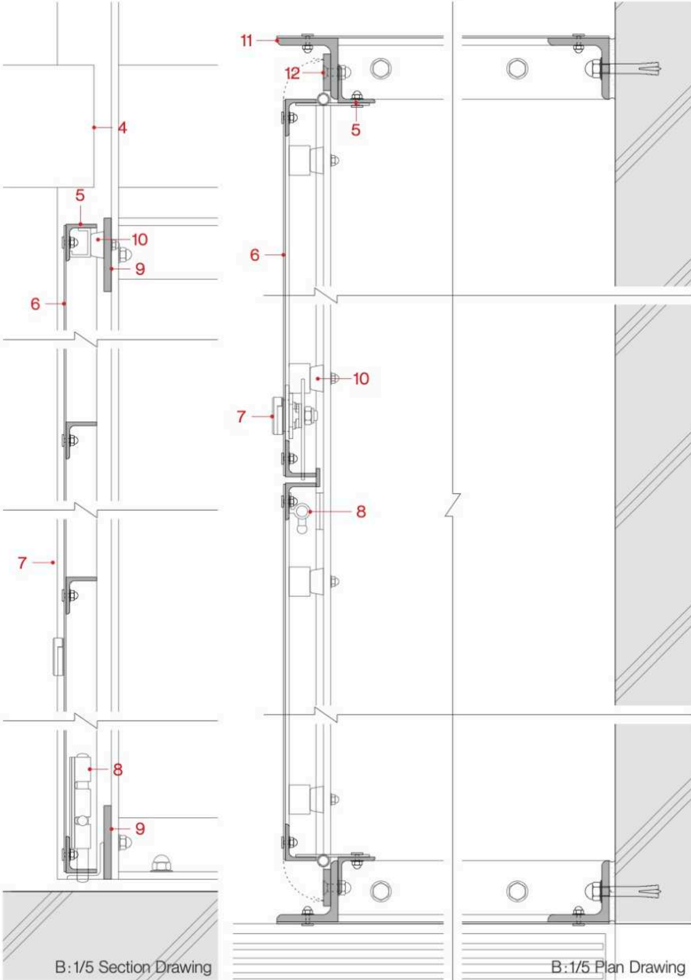
B:1/5 Section Drawing
