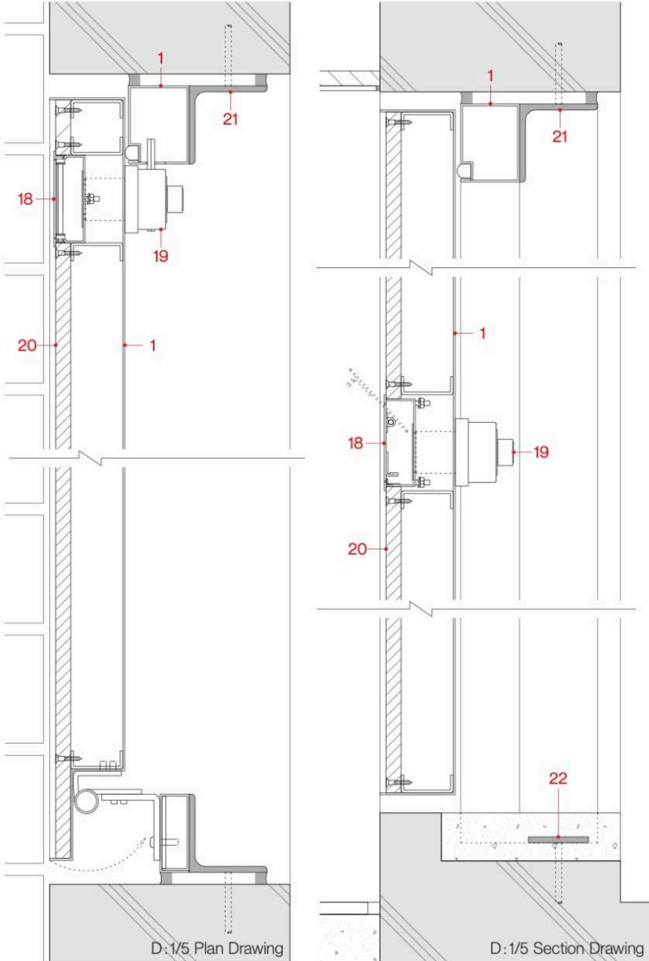
D:1/5 Plan Drawing
