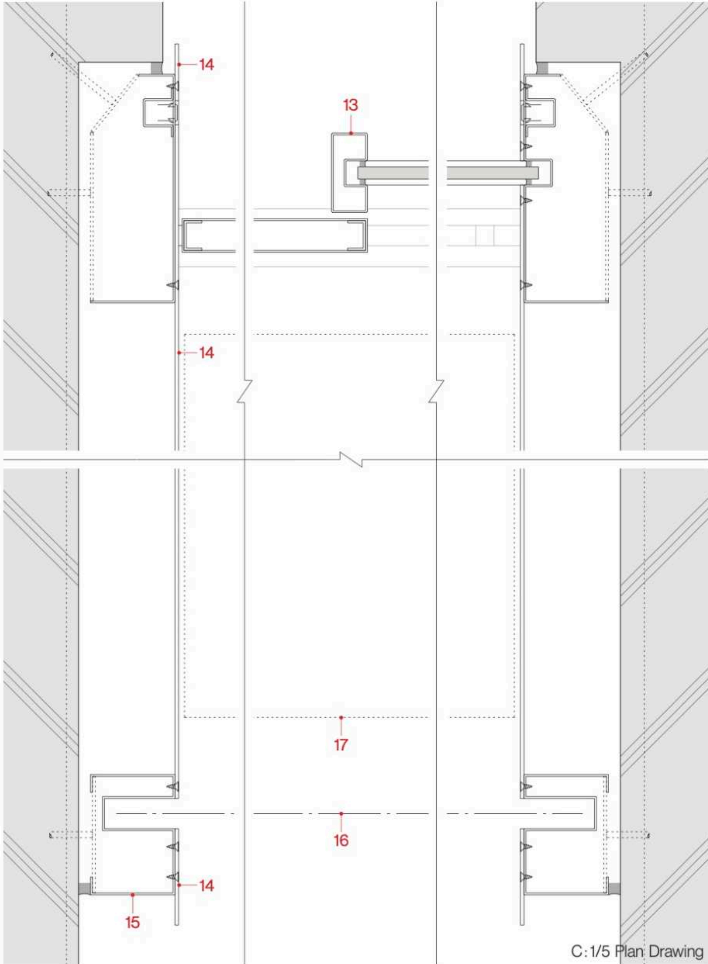
C:1/5 Plan Drawing
