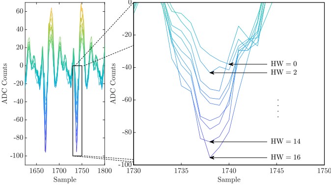
Fig. 4. Leakage for different output HWs of f_{qmul}() at Polars.
