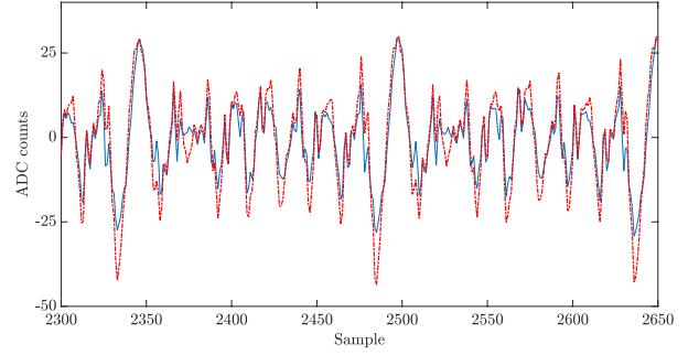
Fig. 14. Average traces: \bar{r}_0 with all-zero message (blue) and \bar{r}_1 with all-one message (red dashed).
