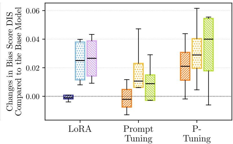
PEFT Method
