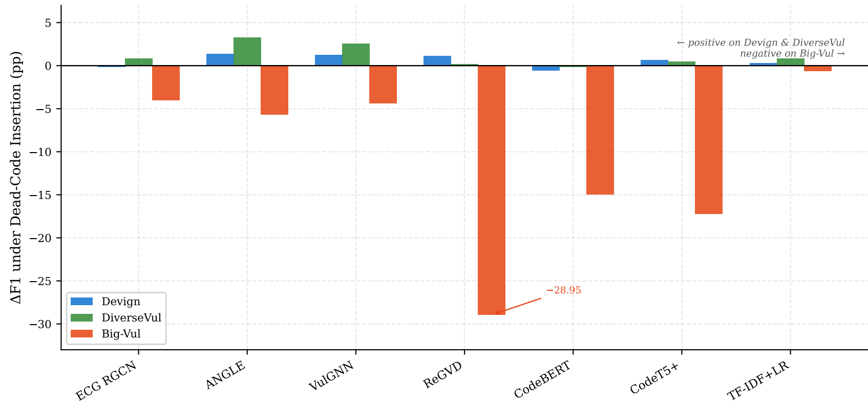
Dead-Code Effect Reverses Across Datasets
