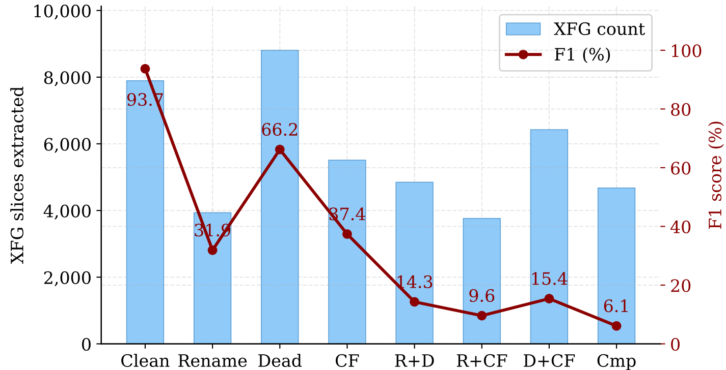
DeepWukong on SARD CWE-119: XFG count and F1 per condition
