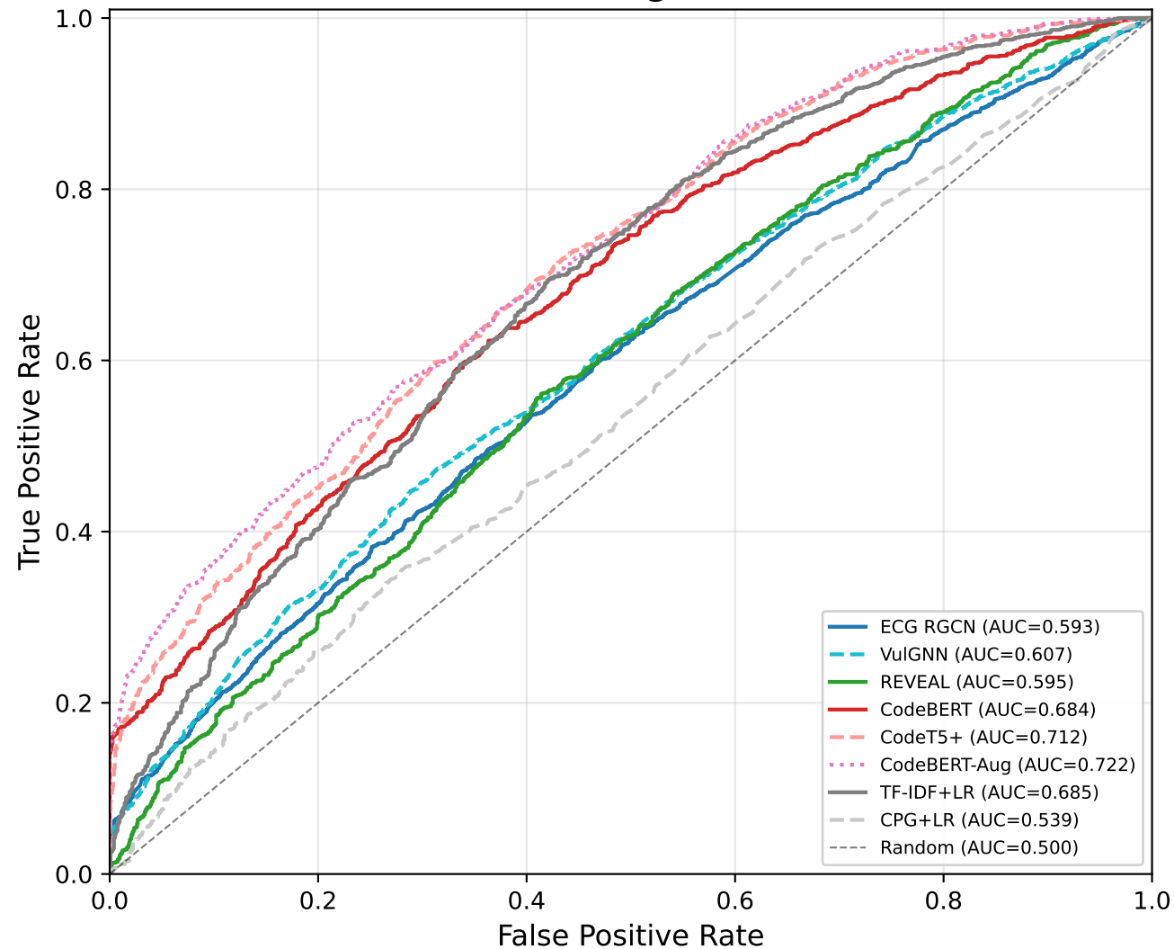
ROC Curves — Design Clean Test Set
