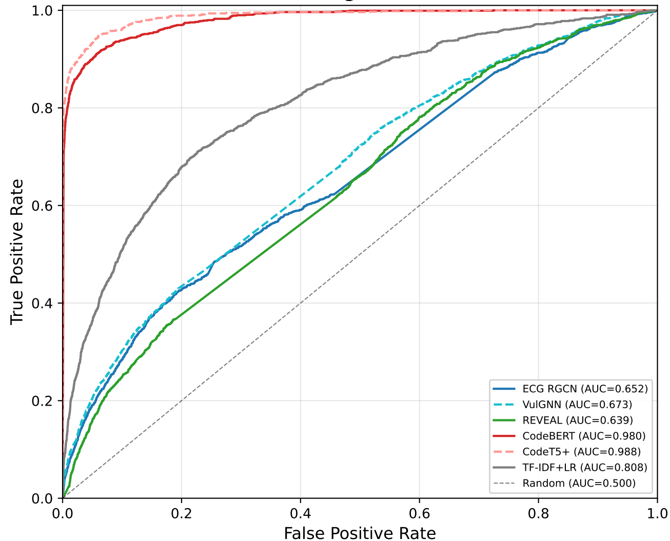
ROC Curves — Big-Vul Clean Test Set
