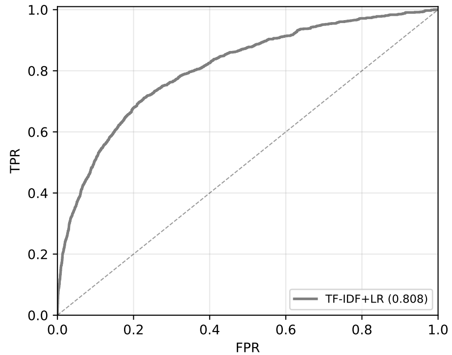
Non-neural
