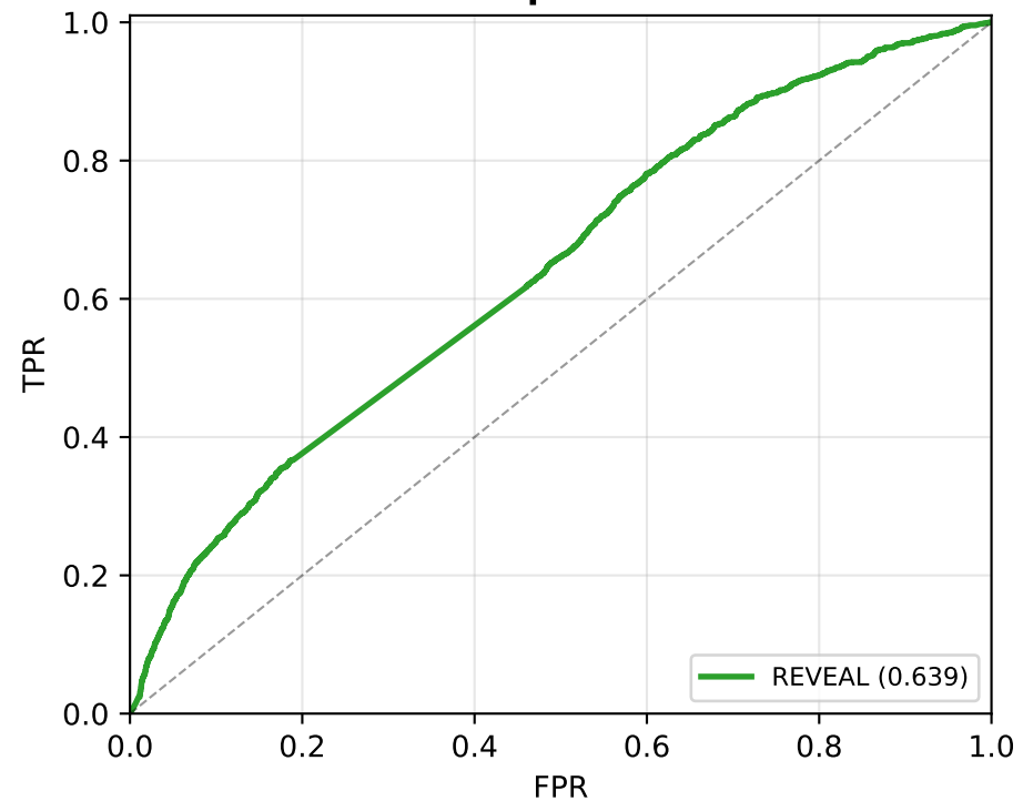
Graph+LM
