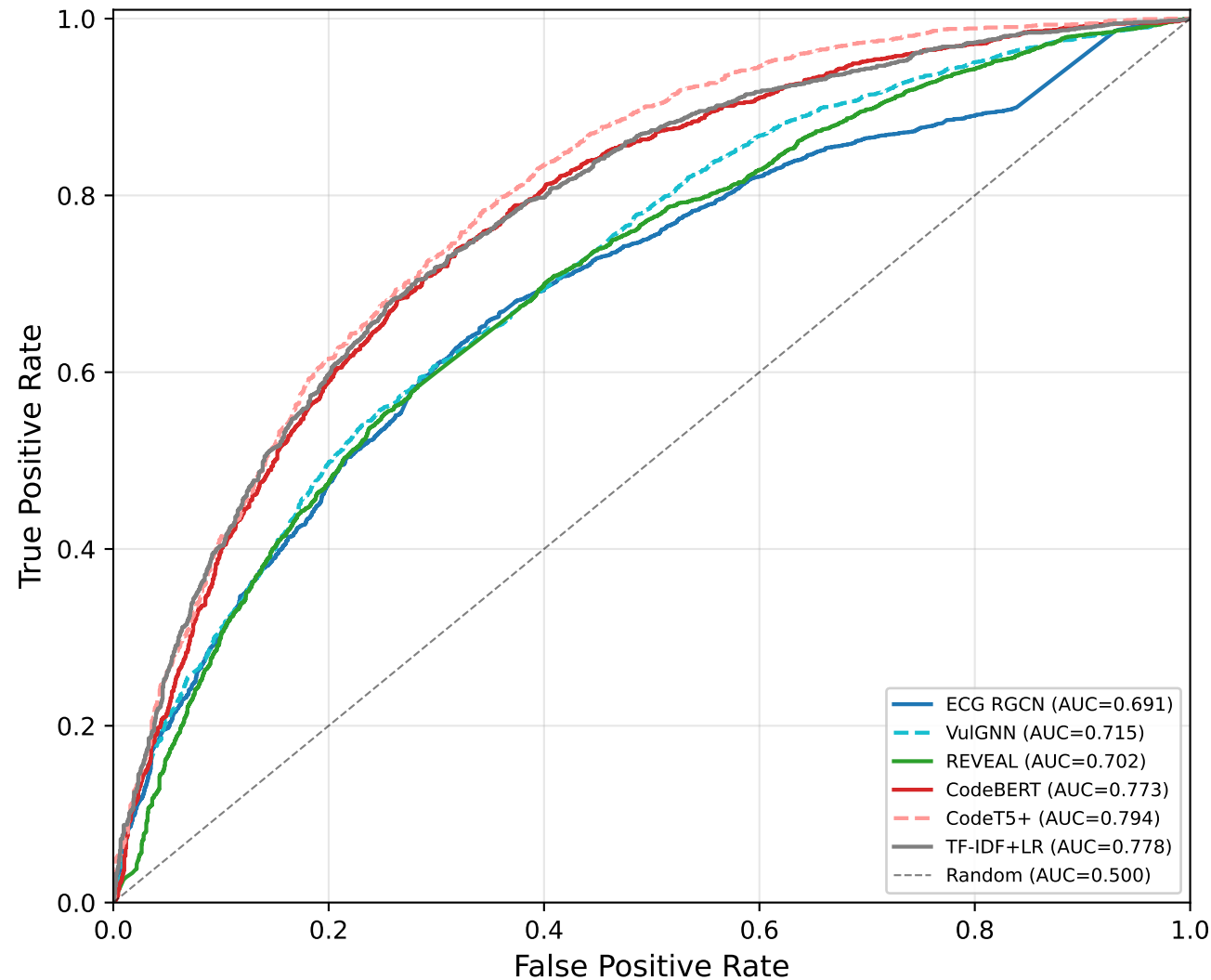
ROC Curves — DiverseVul Balanced Test Set
