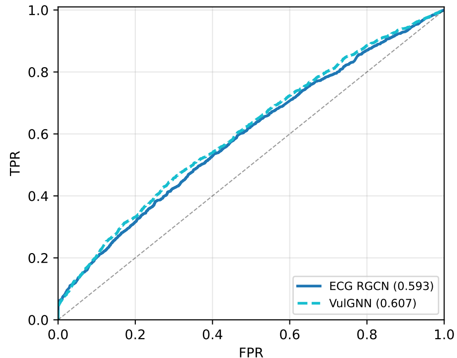
W-GNN
