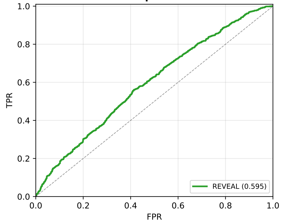
Graph+LM
