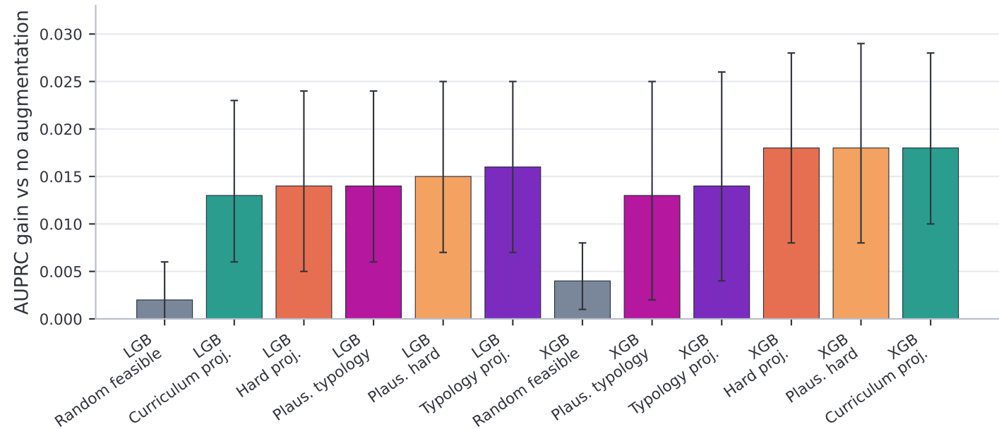
Held-out layering: paired gains by detector and augmentation family
