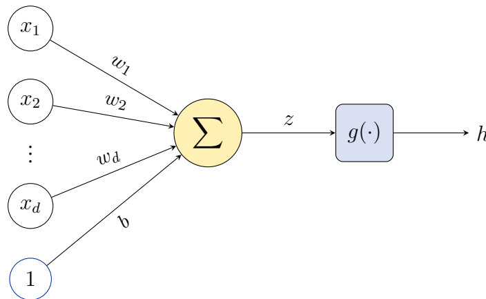
Figure 10.1: A single neuron (perceptron). The inputs x_1, \dots, x_d are combined through the weights w_1, \dots, w_d and a bias b into the linear activation z = w^\top x + b , which the activation function g maps to the output h = g(z) .
