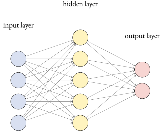
Figure 10.3: A feedforward neural network (multilayer perceptron). Each node is a perceptron unit as in Figure 10.1, organized into layers, with every neuron of one layer feeding into every neuron of the next.
