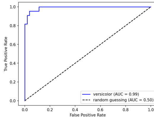
Figure 4.3: ROC curve for the versicolor-vs-rest classifier, with the corresponding AUC compared against random guessing.
