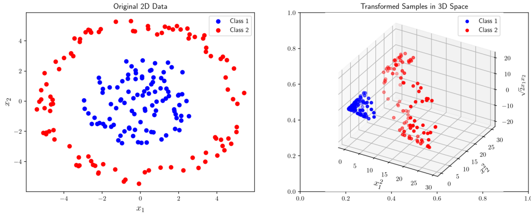
Figure 11.1: Two classes that are not linearly separable in the original 2D input space (left) become linearly separable after the feature transformation \phi(x) = (x_1^2, x_2^2, \sqrt{2}x_1x_2) (right).
