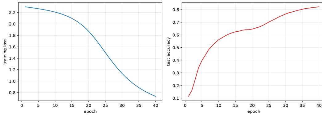
Figure 10.5: Learning curve of the library-based MLP on MNIST: training cross-entropy loss (left) and test accuracy (right) across epochs of plain SGD.
