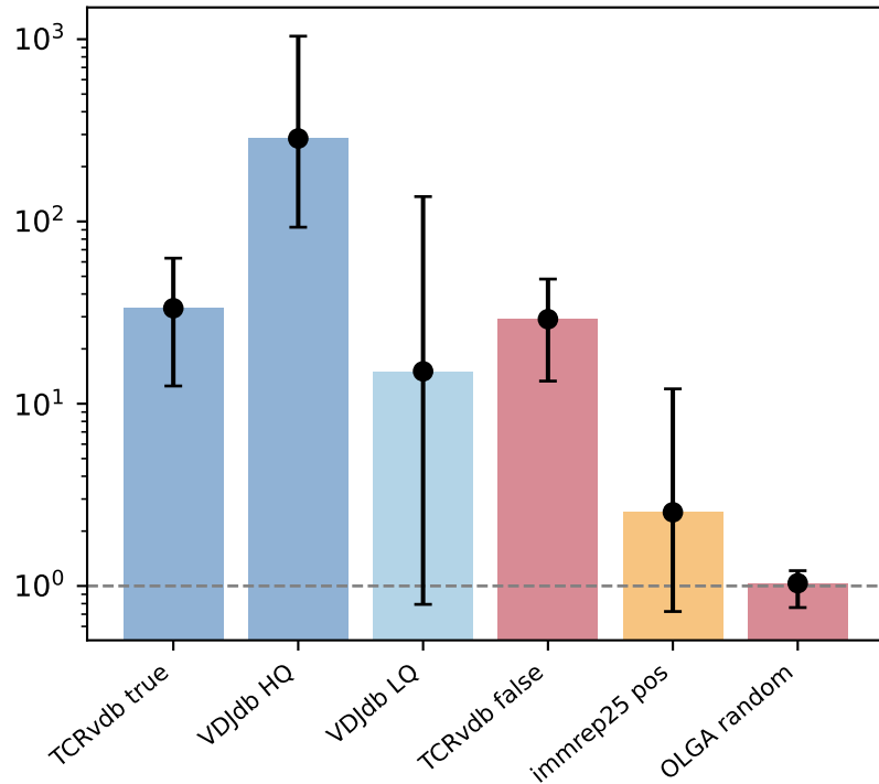
Homology S/N (TRB, d=1)
