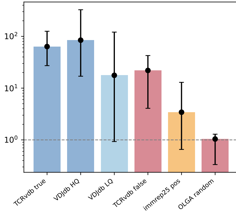
Homology S/N (TRA, d=1)
