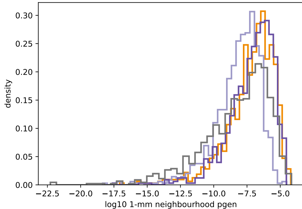
TCR \beta
