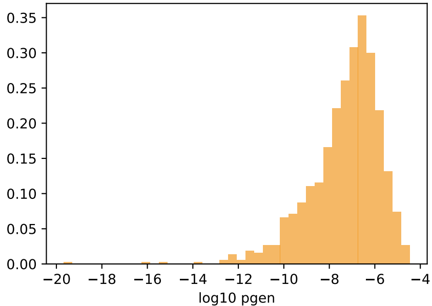
log10 pgen (TRA)
