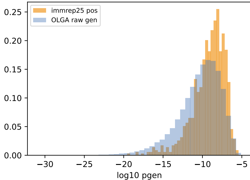
log10 pgen (TRB)
