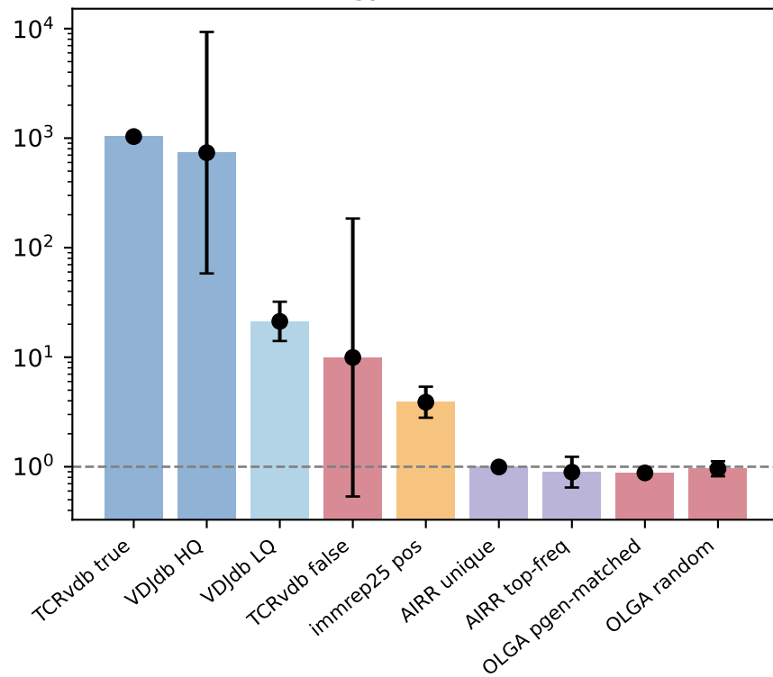
Homology S/N (TRA, d=1)
