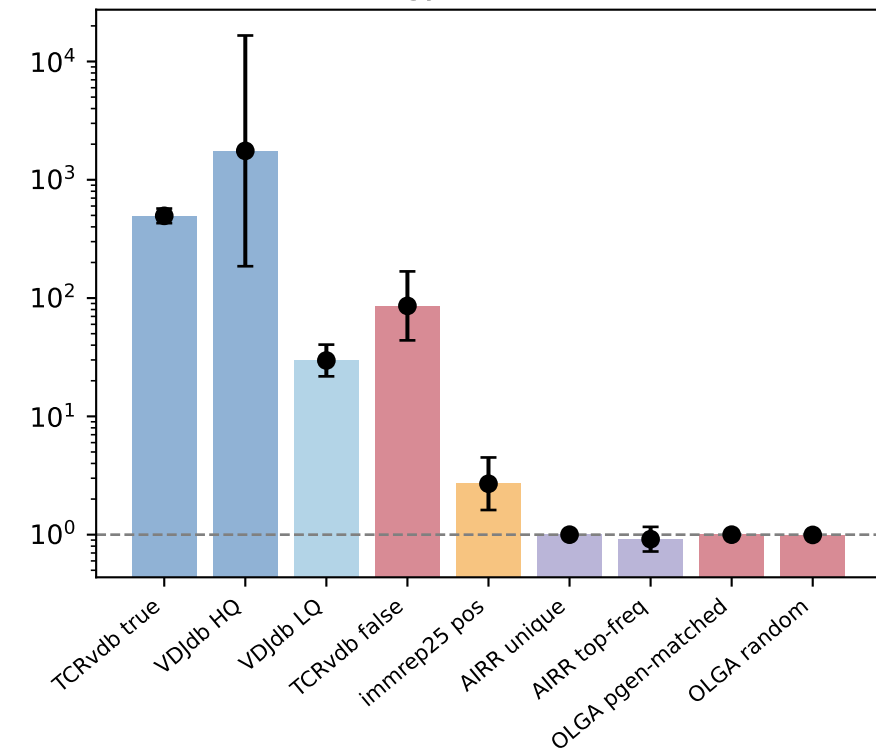
Homology S/N (TRB, d=1)
