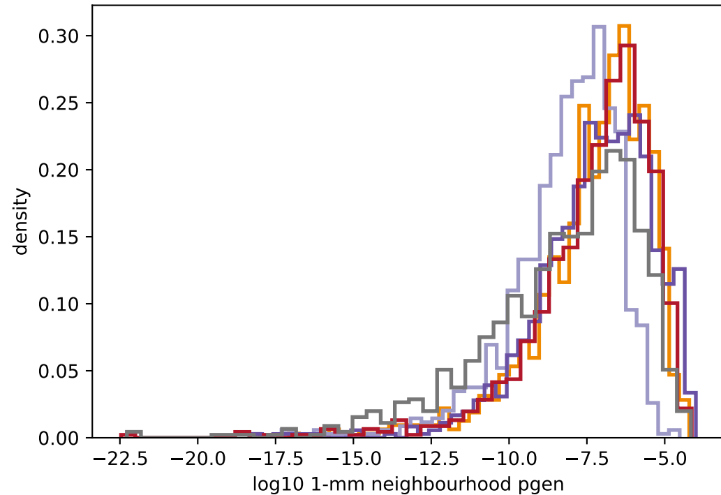
TCR \beta
