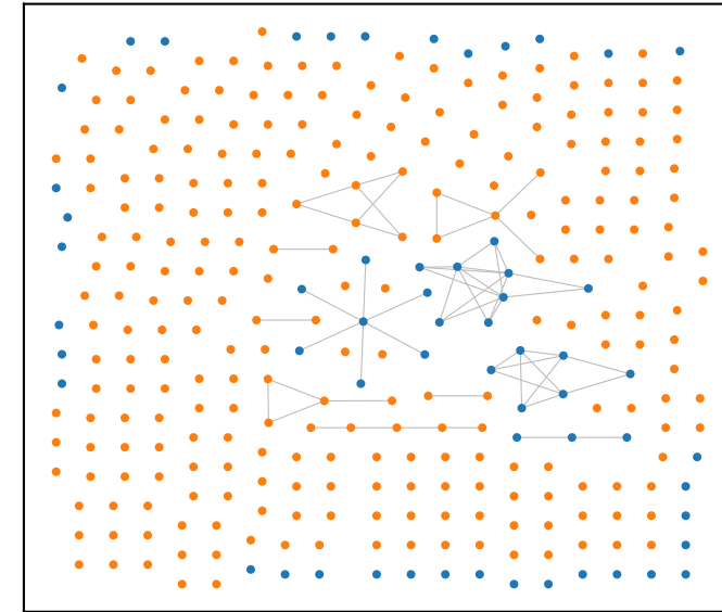
OLGA pgen-ladder (E=20, edges=5)
