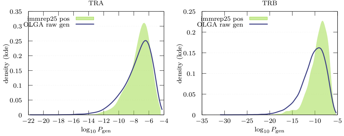
Figure 6: Per-chain \log_{10} P_{\text{gen}} (kernel density): immrep25 positives (filled) vs. raw OLGA generation (line). Positives skew to higher P_{\text{gen}} (public-leaning), motivating the P_{\text{gen}} -matched control.
