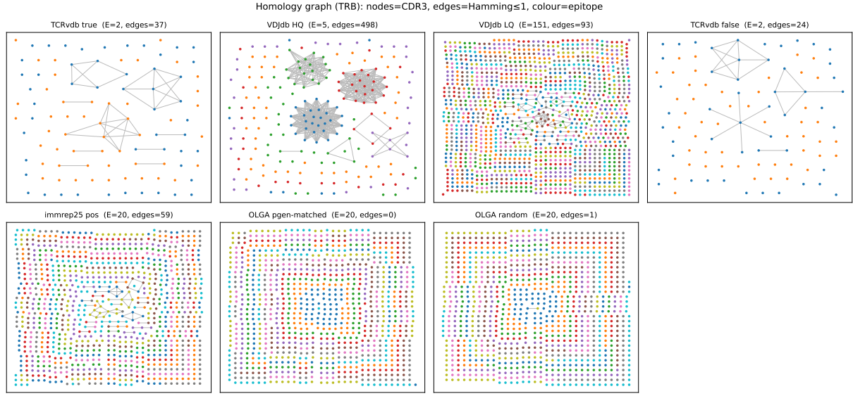
Figure 4: TR \beta homology graph per cohort (all epitopes \geq 30 records). Verified cohorts form dense epitope-coloured cliques; immrep25 and OLGA are near-edgeless.
