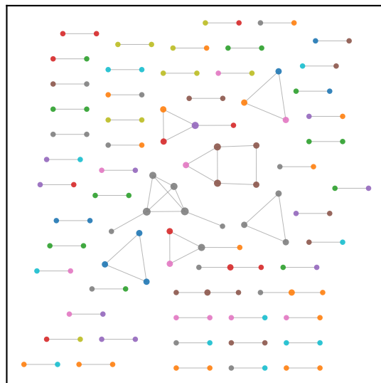
IMMREP25 (+) N =991 receptors, 20 epitopes, 86 edges, 856 with no neighbour (not drawn)
