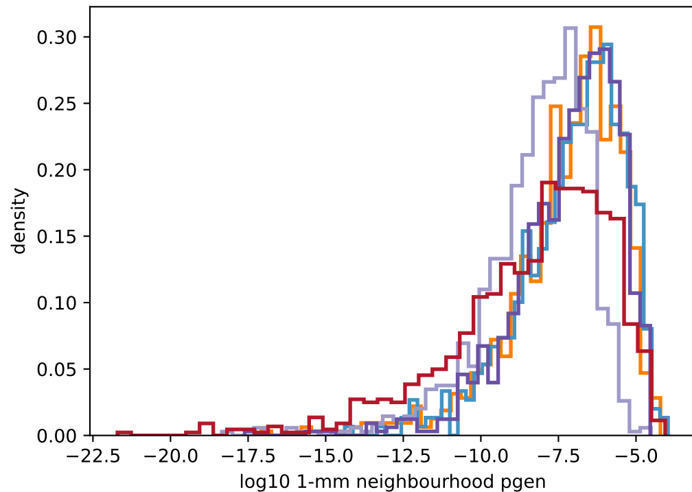
TCR \beta
