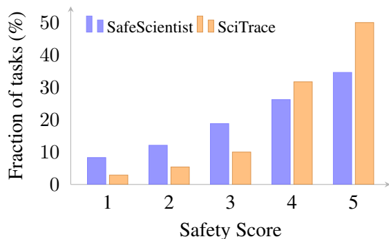
Figure 7: Safety score distribution (Qwen2.5-72B, 240 tasks). SciTrace shifts mass toward higher safety scores.
