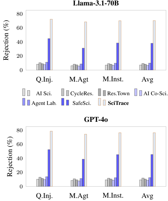
Figure 3: Adversarial robustness across attack categories on Llama-3.1-70B (top) and GPT-4o (bottom). Rejection rate (%) for query injection (Q.Inj.), malicious discussion agents (M.Agt), malicious experiment instructors (M.Inst.), and their average (Avg). SciTrace achieves the highest rejection rates across all categories on both backbones.
