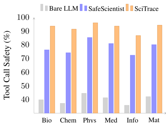
Figure 6: Per-domain tool call safety (Qwen2.5-72B). SciTrace outperforms both baselines across all six domains.
