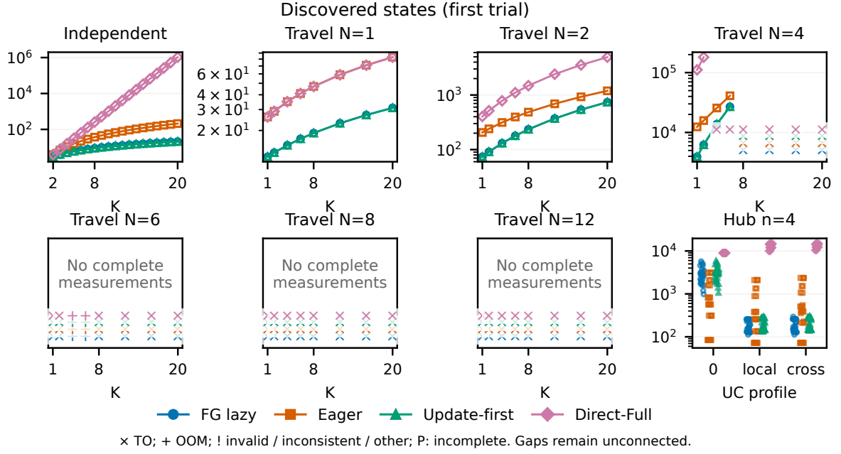
Figure S2: Full scaling-state panels, retaining every tested Travel concurrency level and every hub profile. RQ4 is the archived campaign name; these results appear under RQ3 in the main paper. The saved plots label the independent component count as K ; it is n in the main paper and S2, distinct from Travel's choice count K . Censored outcomes have status marks and no numeric ordinate.
