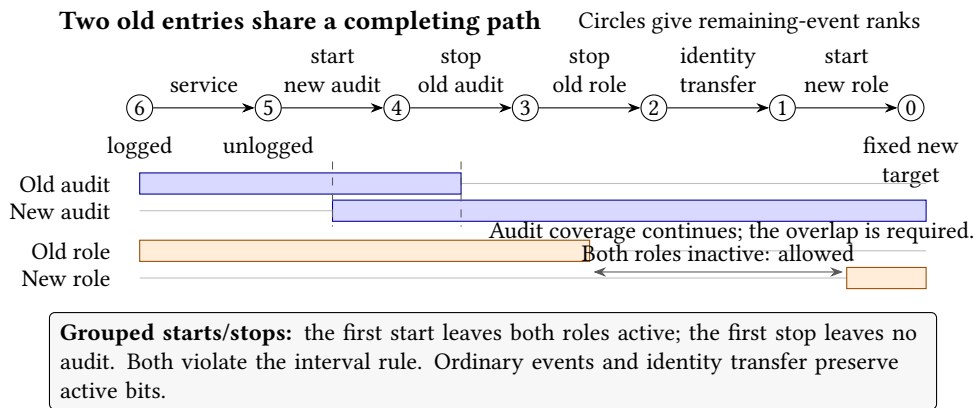
Figure A3: A saved Policy certificate with no supplied precedence; ranks need not be shortest. Logged/unlogged mark both entries; bars mark active requirements. New-audit start resets to unlogged; handover reaches new audit unlogged and new role valid. Arrows have one action and outcome. The role gap is allowed; ordinary events may be withheld, with no service-continuity guarantee.
