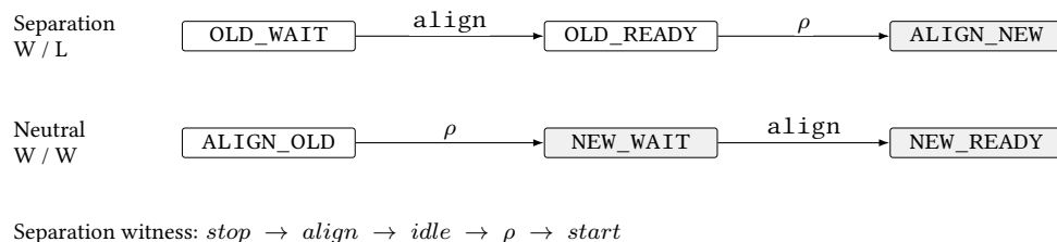
Figure S2: Measured requirement-boundary inputs. Row outcomes are free/block (W: WIN, L: LOSS). All events are controllable; shaded states are new. Each node has an idle loop; neutral also has bad loops. \rho is the sole transfer. Old/new monitors forbid align in separation and bad in neutral. An interval monitor permits start only after align since entry. A requirement block forbids intervening events/transfers between stop and start . Separation is WIN with free boundaries and LOSS with a block; neutral is WIN in both.
