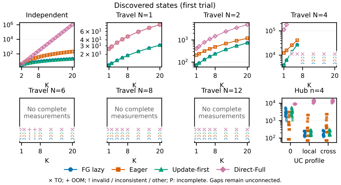
Figure S3: Full scaling-state panels, retaining every tested Travel concurrency level and every hub profile. RQ4 is the archived campaign name; these results appear under RQ3 (Scaling limits) in the main paper. The saved plots label the independent component count as K ; it is n in the main paper and S2, distinct from Travel's choice count K . Censored outcomes have status marks and no numeric ordinate.
