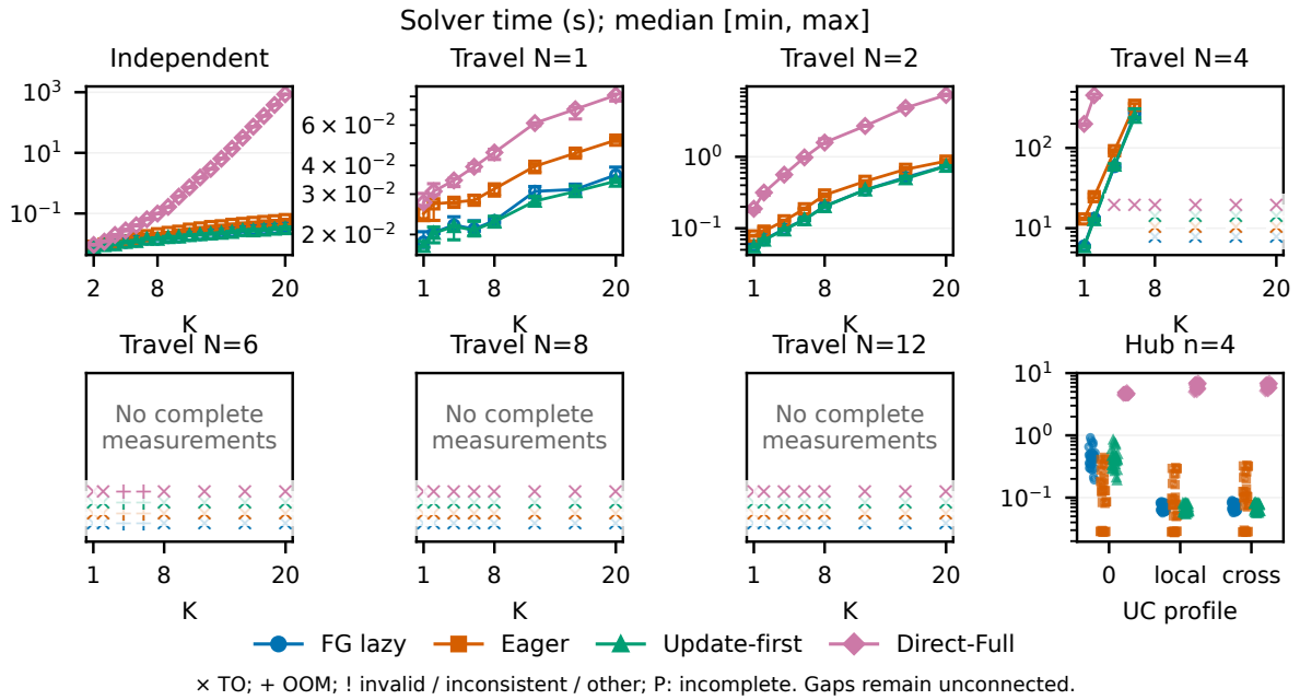
Figure S2: Full scaling-time panels from the archived RQ4 campaign. Medians and ranges require five valid, consistent completions; TO/OOM and other incomplete outcomes remain visible.
