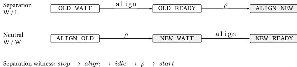
Figure S1: Measured requirement-boundary inputs. Row outcomes are free/block (W: WIN, L: LOSS). All events are controllable; shaded states are new. Each node has an idle loop; neutral also has bad loops. \rho is the sole transfer. Old/new monitors forbid align in separation and bad in neutral. An interval monitor permits start only after align since entry. A requirement block forbids intervening events/transfers between stop and start . Separation is WIN with free boundaries and LOSS with a block; neutral is WIN in both.
