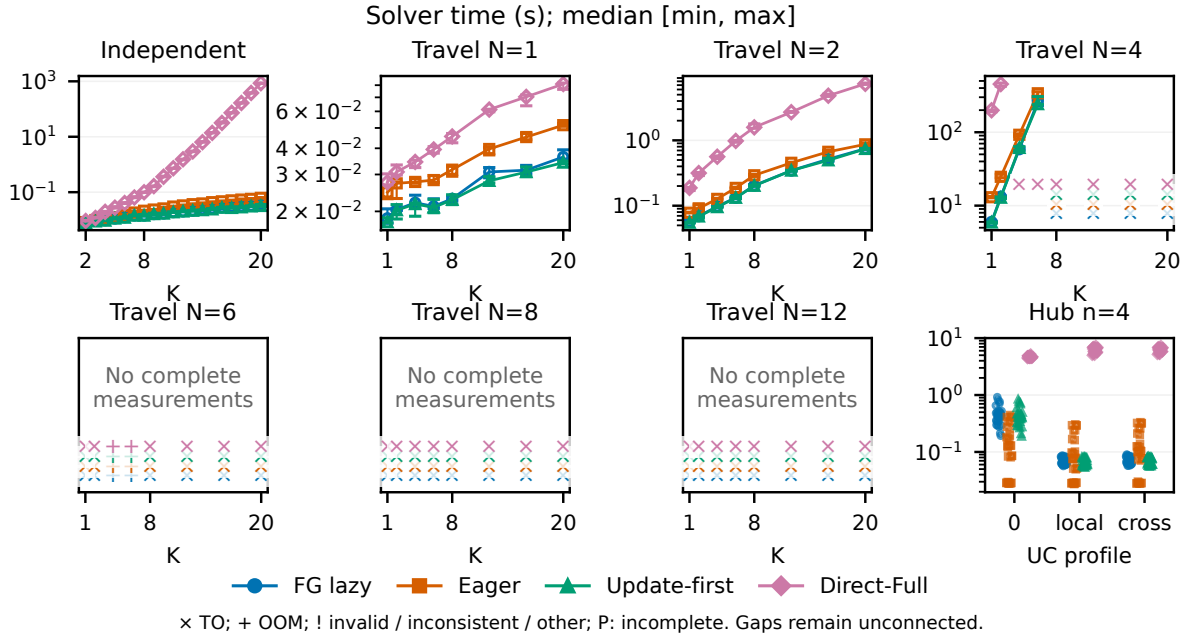
Figure S3: Full scaling-time panels from the archived RQ4 campaign. Medians and ranges require five valid, consistent completions; TO/OOM and other incomplete outcomes remain visible.
