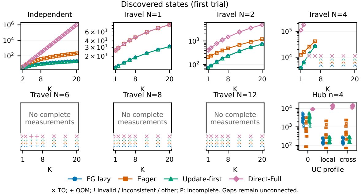
Figure S2: Full scaling-state panels, retaining every tested Travel concurrency level and every hub profile. RQ4 is the archived campaign name; these results appear under RQ3 (Scaling limits) in the main paper. The saved plots label the independent component count as K ; it is n in the main paper and S2, distinct from Travel's choice count K . Censored outcomes have status marks and no numeric ordinate.
