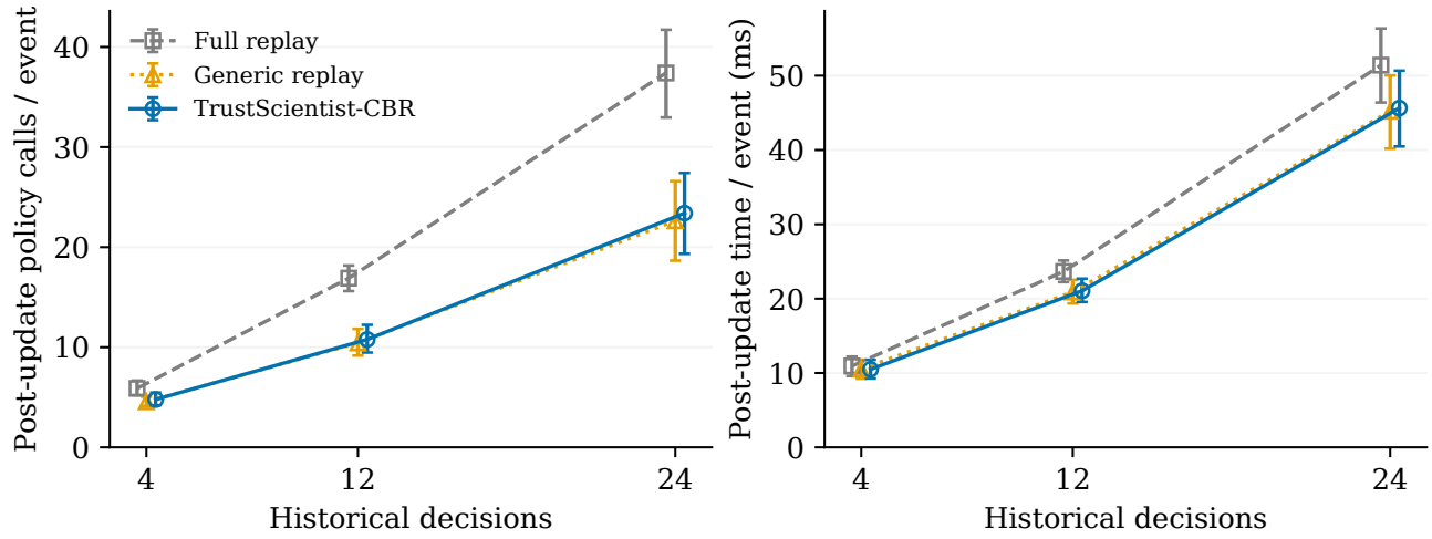
Figure 7: Work and measured time on executed scripted histories. Each length contains 72 paired events (controlled updates) on 12 dataset-split clusters. Policy calls include re-audit, receipt verification and continuation. Horizontal offsets separate overlapping methods. Only the three methods with consistent final outputs on all episodes are shown. Points are means; whiskers are 95% cluster-bootstrap intervals. Time uses two balanced repetitions of the same cases. Common initialization is excluded; continuation includes actual model refits. Generic replay matches correctness and uses fewer policy calls than CBR.
