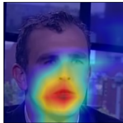
Q70 acc. 0.650
