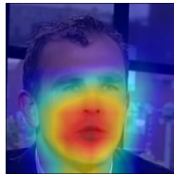
Q50 acc. 0.536
