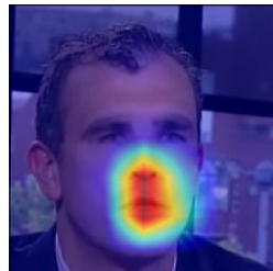
Q50 acc. 0.666
