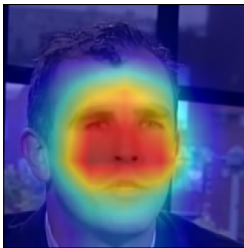
Original acc. 0.944
