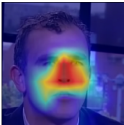
Original acc. 0.953
