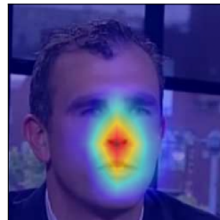
Q30 acc. 0.555
