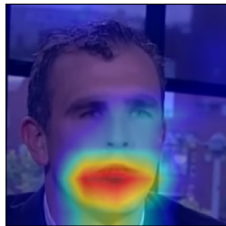
Q90 acc. 0.839
