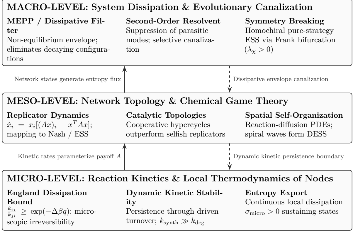
Figure 2: The three-level hierarchical cascade of Functional Stability Theory II (FST-II), detailing the upward kinetic-to-dissipation parameterization and the downward stability constraints connecting microscopic non-equilibrium thermodynamics, mesoscopic chemical game theory, and macroscopic dissipative canalization.
