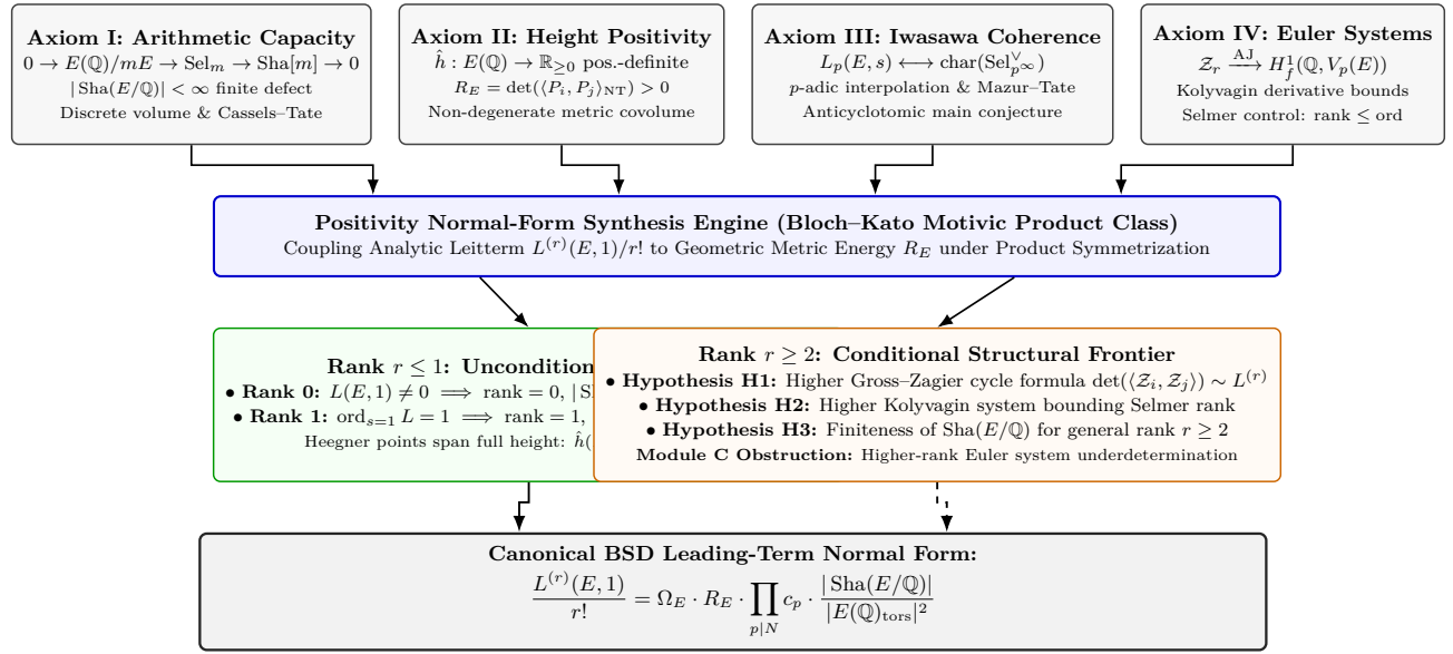
FIG. 1. The 4-axiom positivity architecture and modular flow of the Birch and Swinnerton-Dyer normal-form framework. Top: The four foundational building blocks (Axiom I arithmetic capacity, Axiom II Néron–Tate quadratic energy, Axiom III Iwasawa composition coherence, and Axiom IV Euler system derivative bounds). Center: The synthesis engine within the Bloch–Kato motivic product class. Bottom: Epistemological bifurcation into the unconditional rank r \leq 1 theorems (Gross–Zagier, Kolyvagin, Kato) and the conditional higher-rank structural frontier ( r \geq 2 ), culminating in the canonical BSD leading-term normal form.
