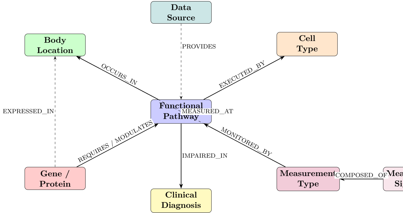
Figure 1: Entity-relationship diagram of the pathway-centric knowledge graph. Solid arrows indicate primary relationships through the pathway hub; dashed arrows indicate secondary cross-links.
