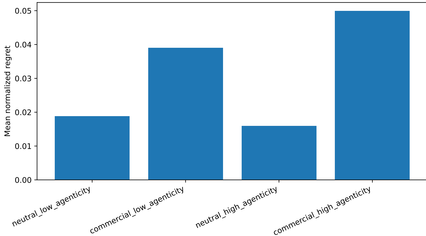
Figure 4 — Normalized utility regret by condition
