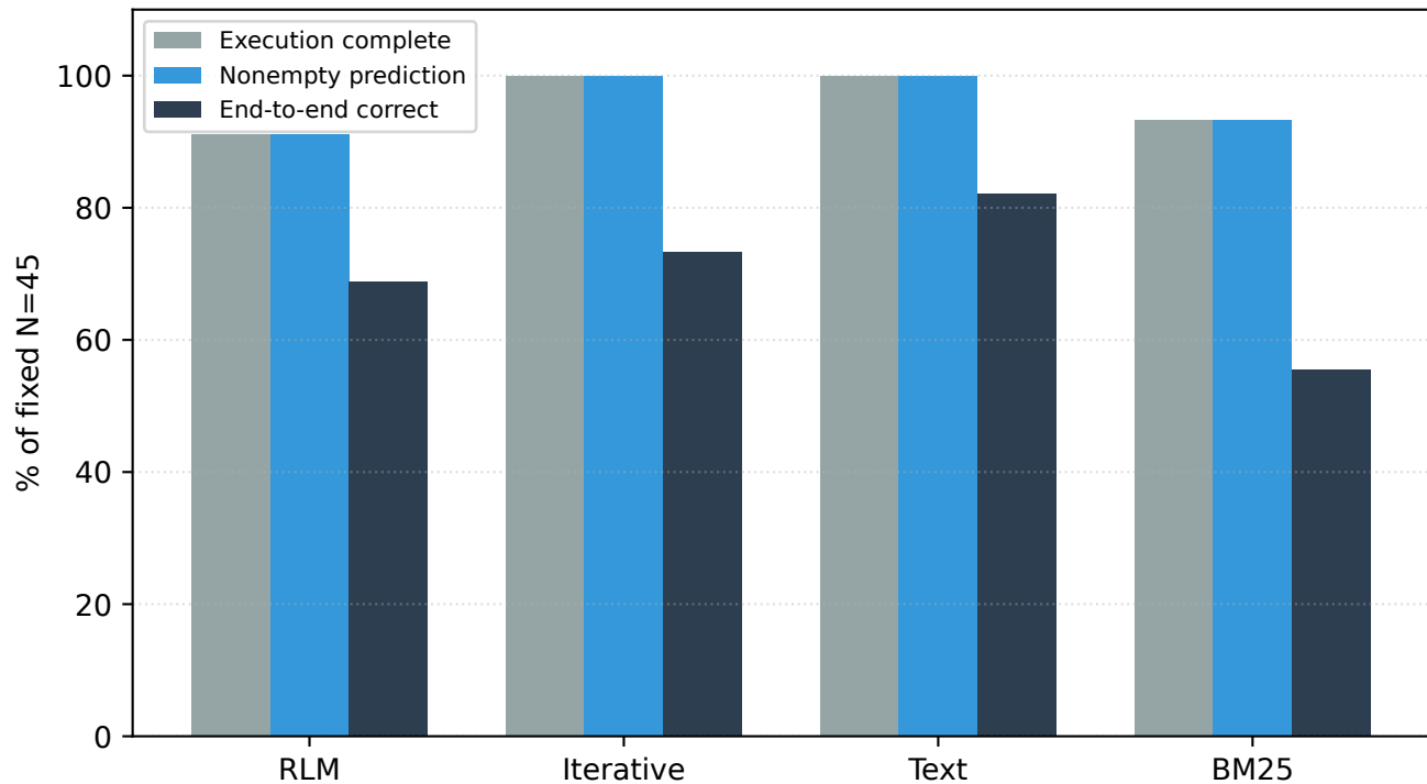
Completion vs correctness decomposition (seed-20)
