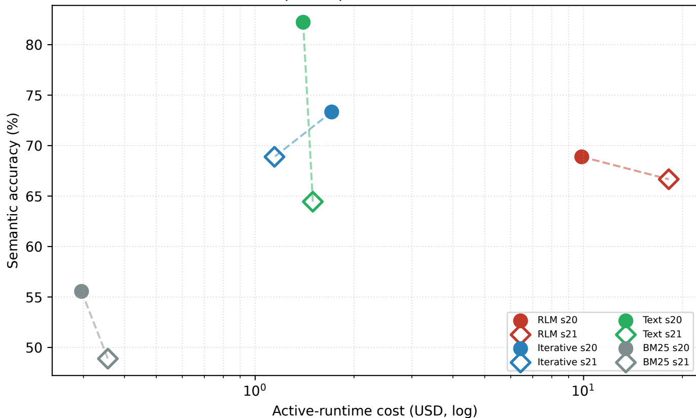
Route movement across equal-cap rollouts (filled: seed 20; hollow: seed 21)
