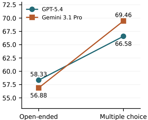
(b) SDABench: SDA-Synth
