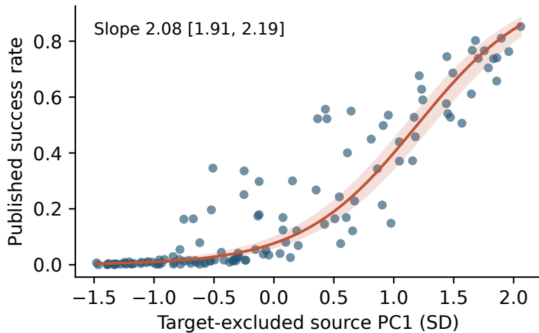
GSM8K: 124 models, 39 families
