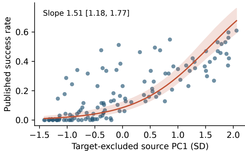
HumanEval: 124 models, 39 families
