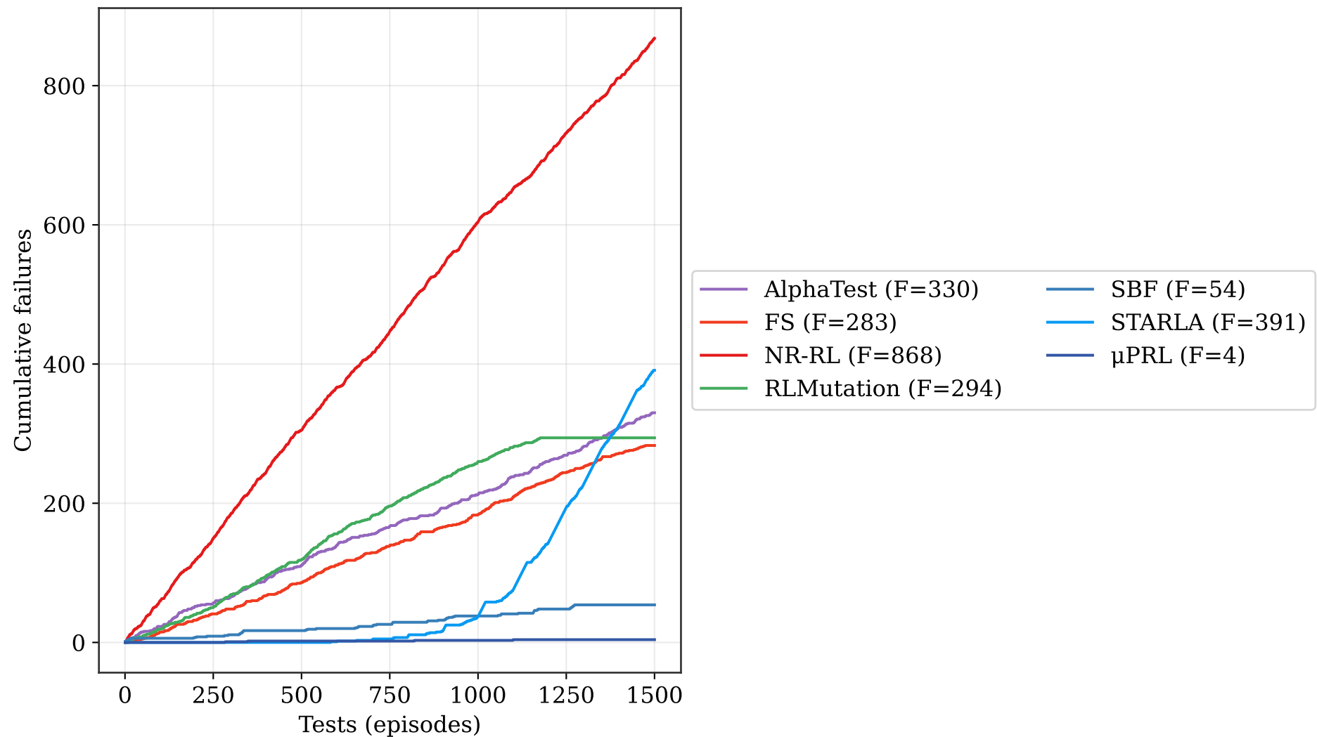
Taxi — Cumulative Failures vs Tests
