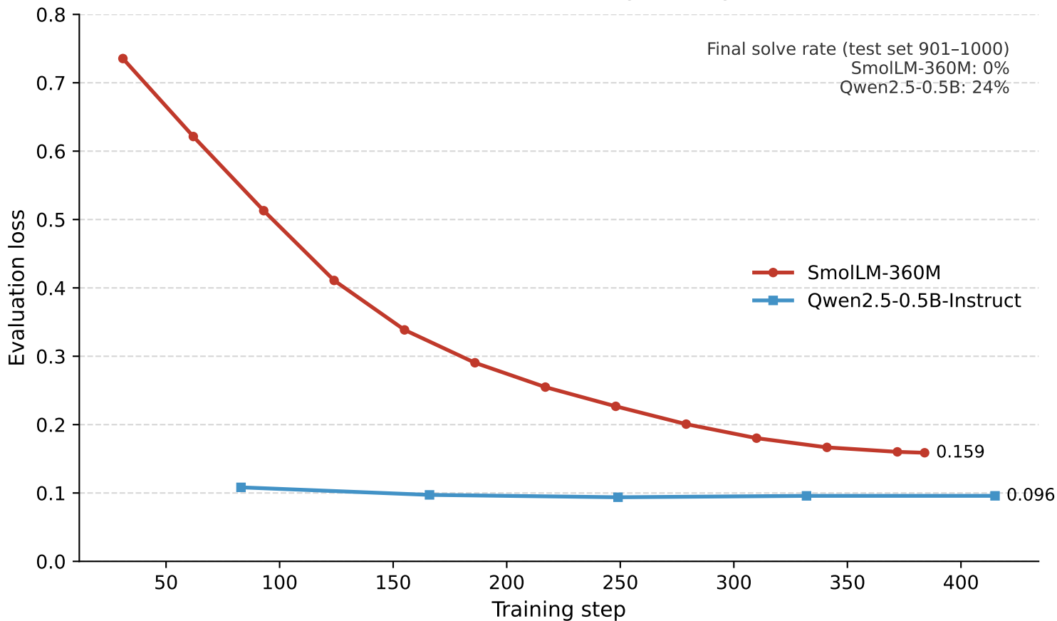
Evaluation loss during training
