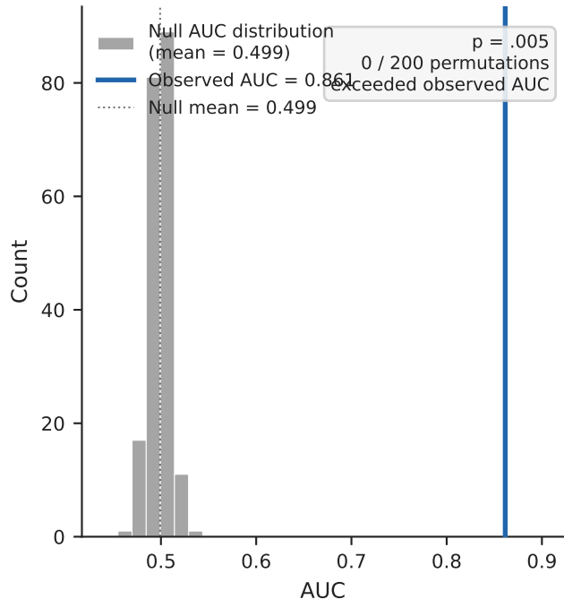
Permutation Test (within-subject label shuffling)
