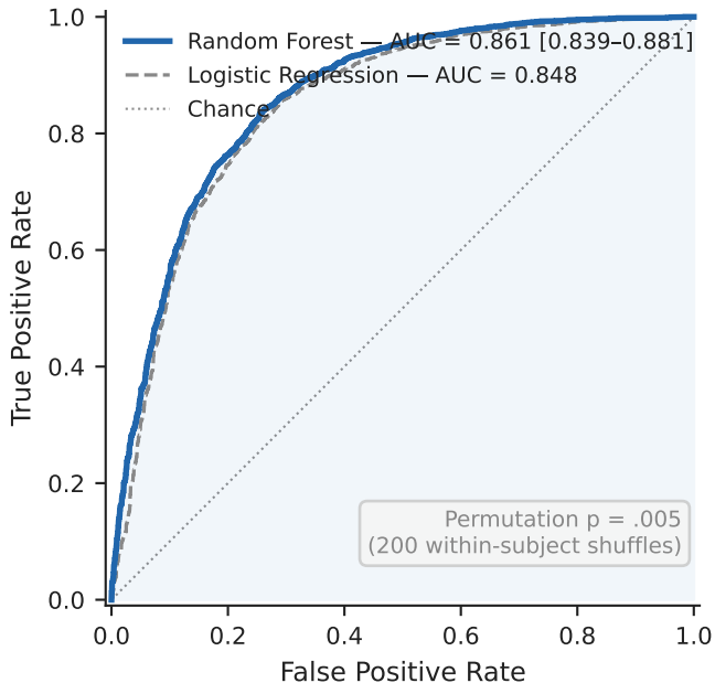
ROC Curve — LOSO Cross-Validation (83 subjects, 5,609 trials)
