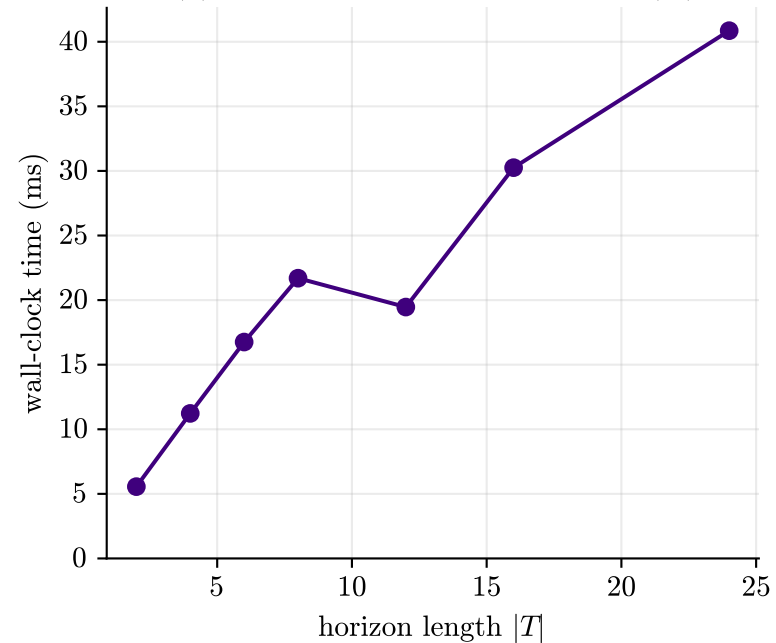
(c) exact DP at n = 12 against |T|
