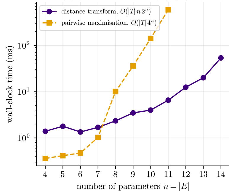
(a) exact DP over \mathcal{P}(E) , |T| = 6
