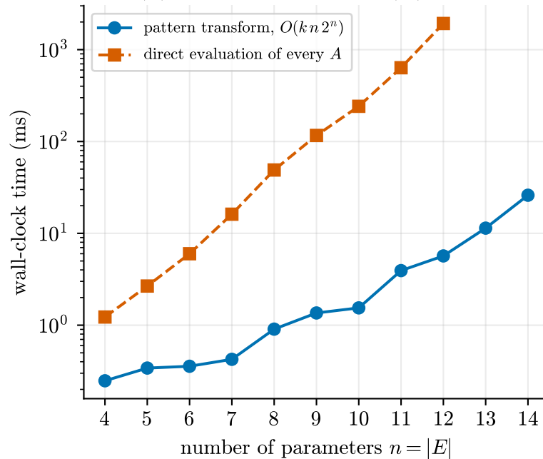
(b) tabulating Q_t on \mathcal{P}(E) , k = 3
