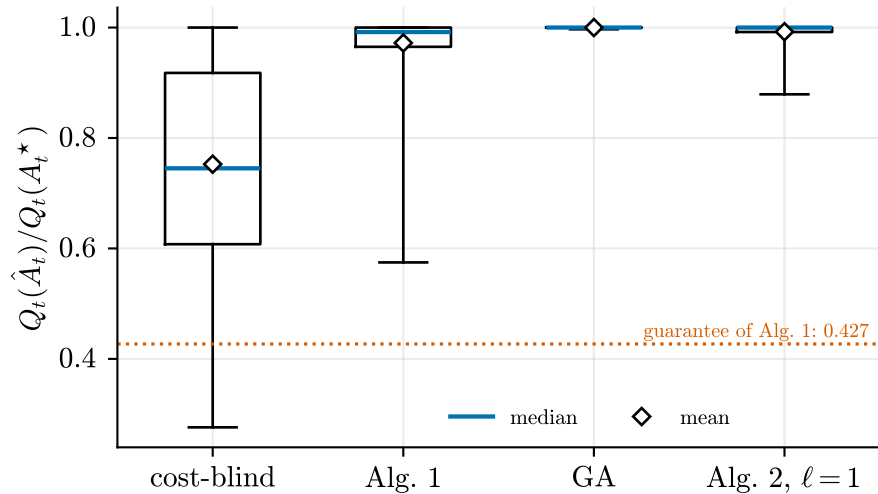
(b) attained fraction of Q_t(A_t^*)
