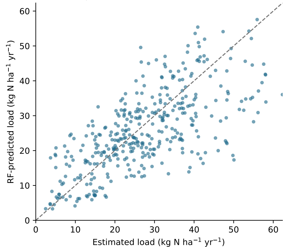
(a) Temporal hold-out: NSE=0.41, KGE=0.65
