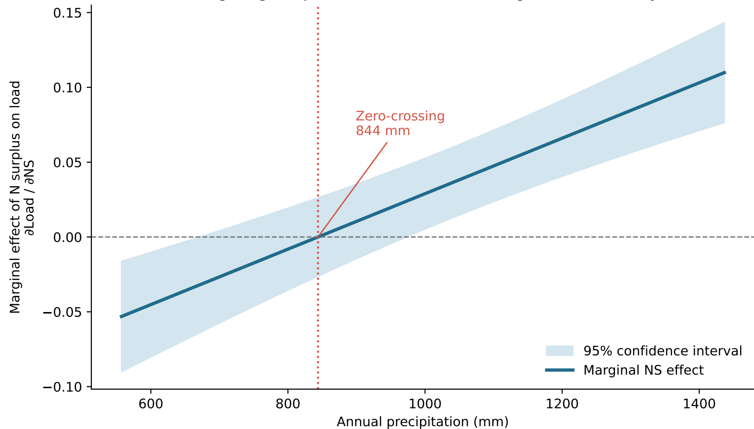
Climate gating: surplus-load association strengthens in wetter years
