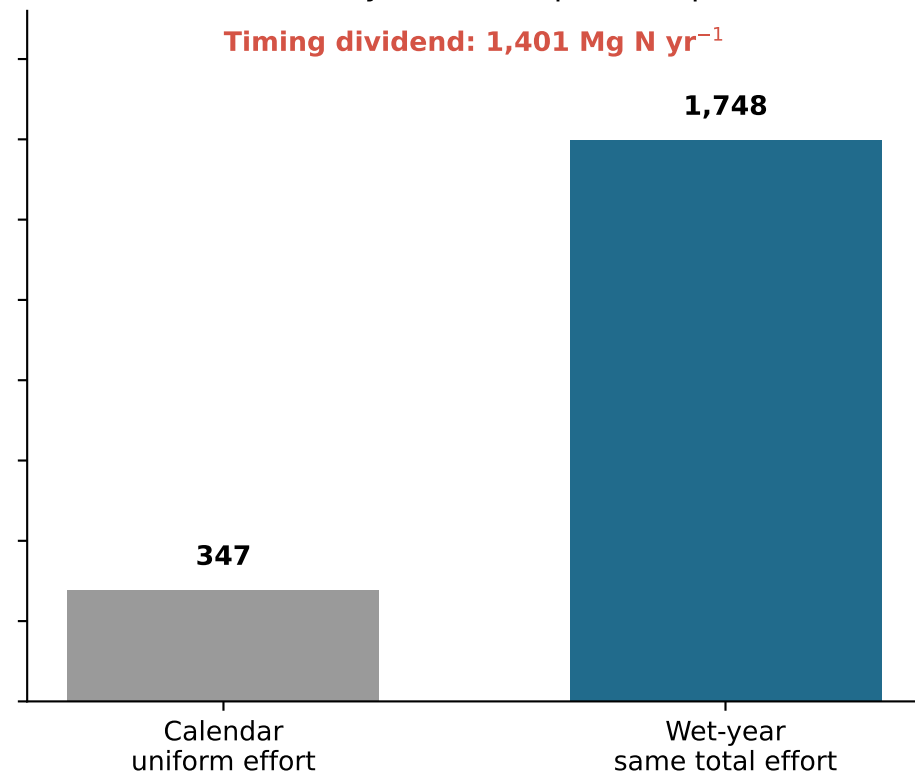
(b) Sensitivity: model-implied response
