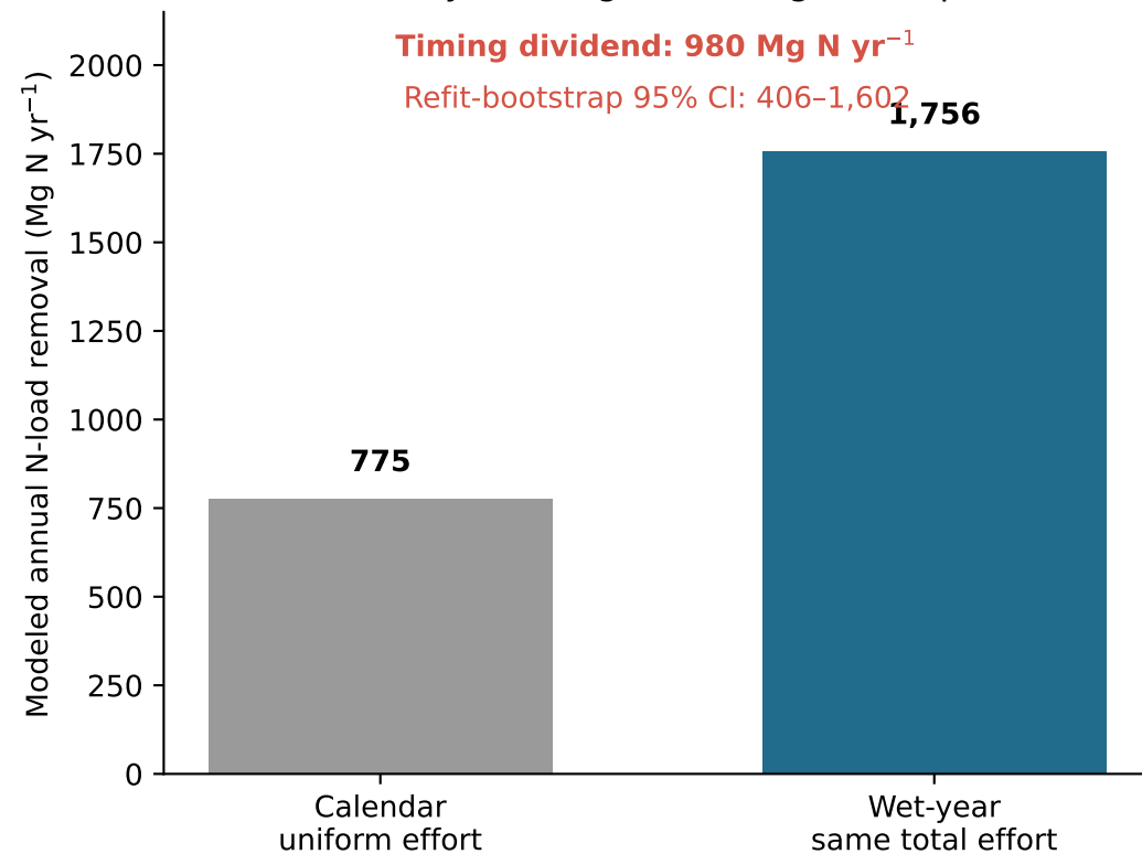
(a) Primary: nonnegative marginal response
